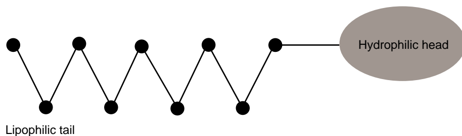
Figure 2. Polliwog representation of a surfactant molecule
